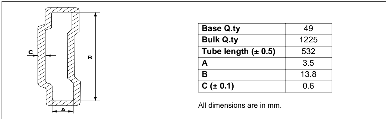
Figure 34. PowerSSO-24 Tube Shipment (No Suffix)
