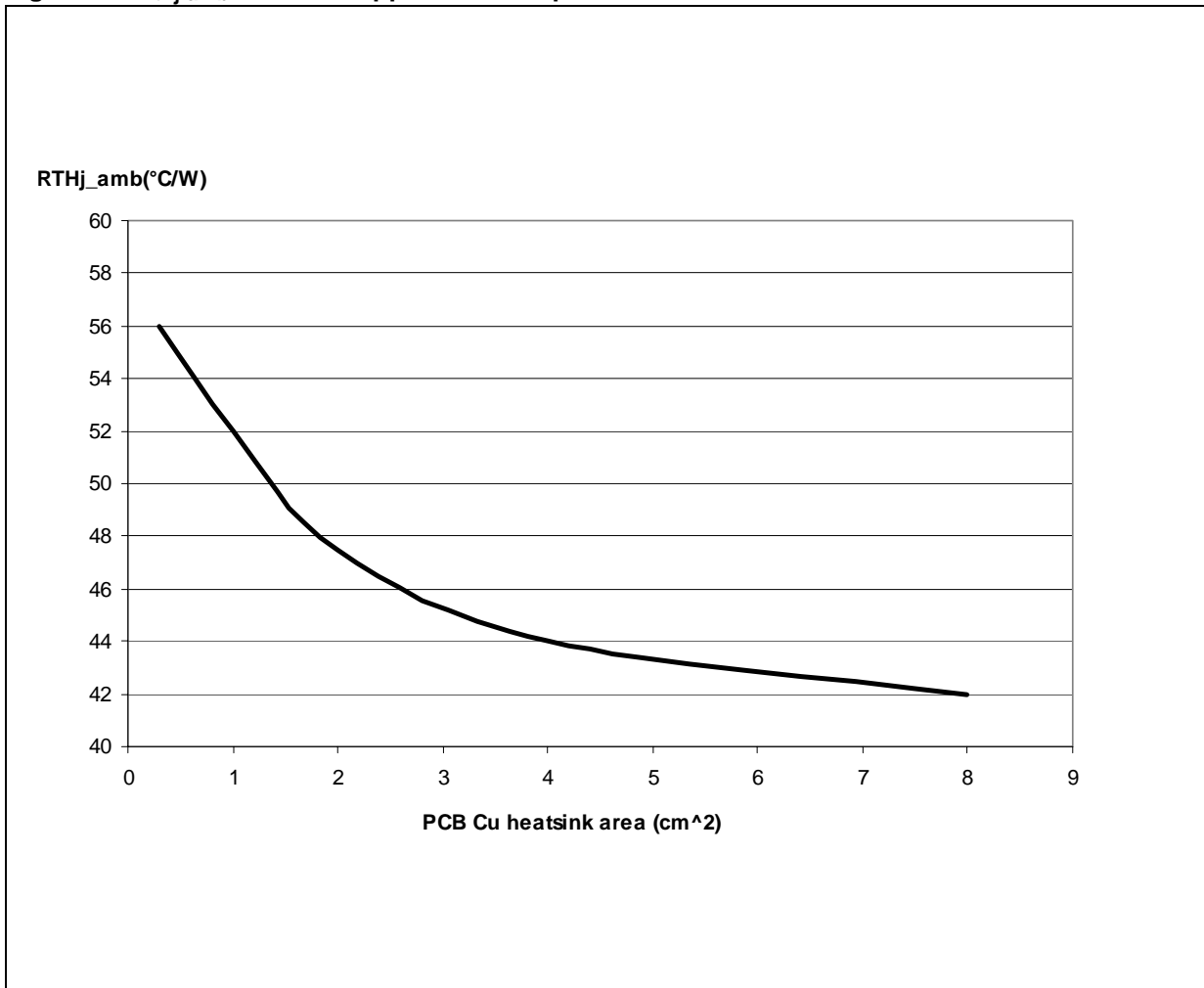
Figure 30. R_{thj-amb} Vs PCB Copper Area in Open Box Free Air Condition
