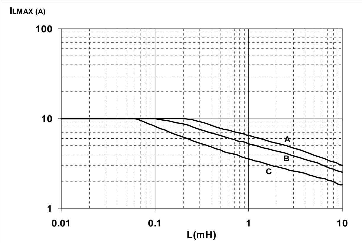
Figure 28. Maximum Turn Off Current Versus Load Inductance
