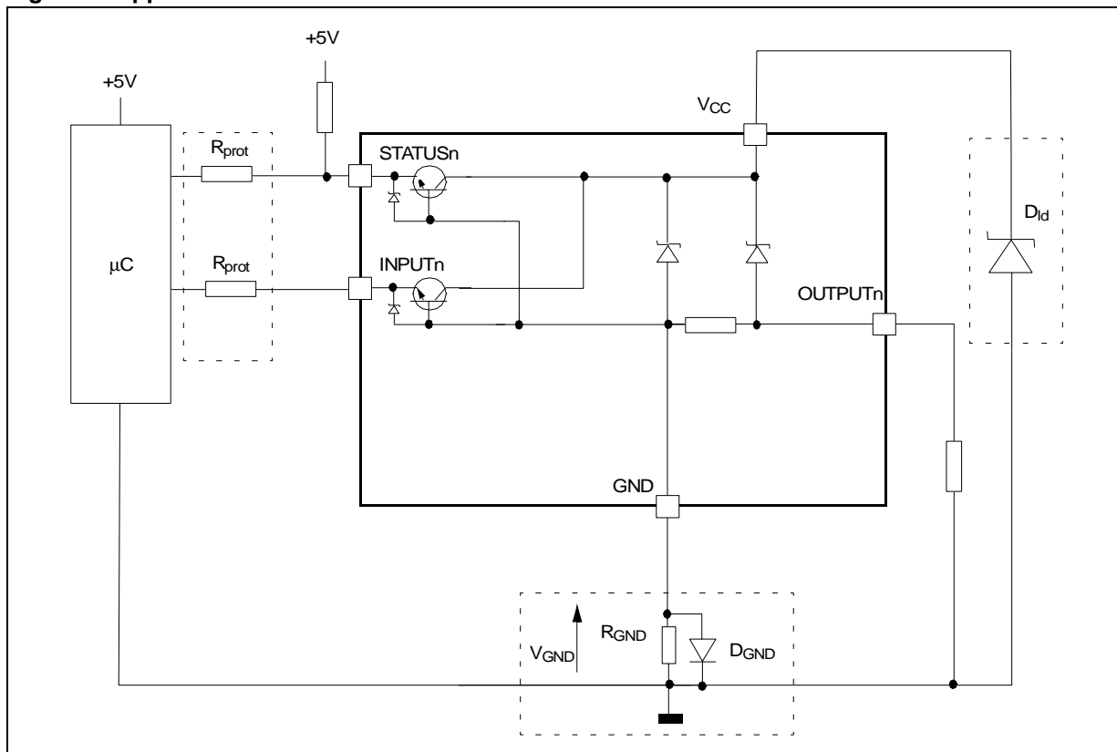
Figure 7. Application Schematic
