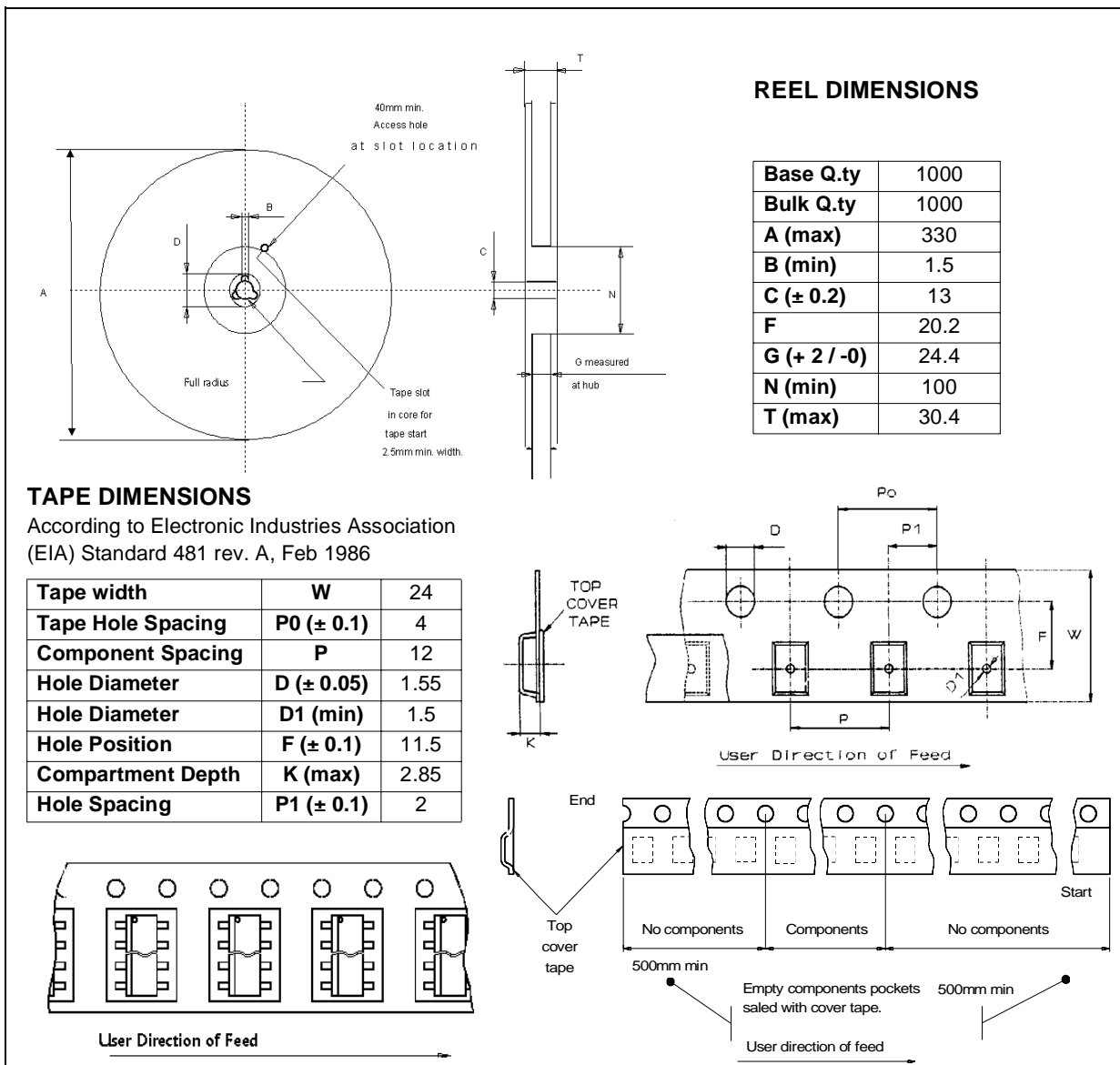
Figure 35. Tape And Reel Shipment (Suffix "TR")
