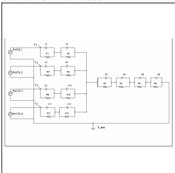
Figure 32. Thermal Fitting Model of a Quad Channel HSD in PowerSSO-24
