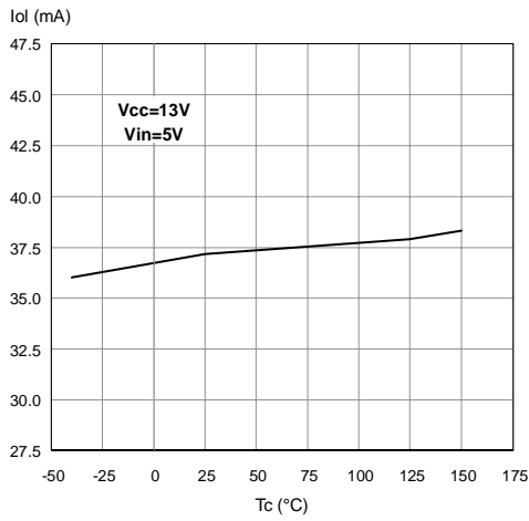
Figure 22. Openload On State Detection Threshold
