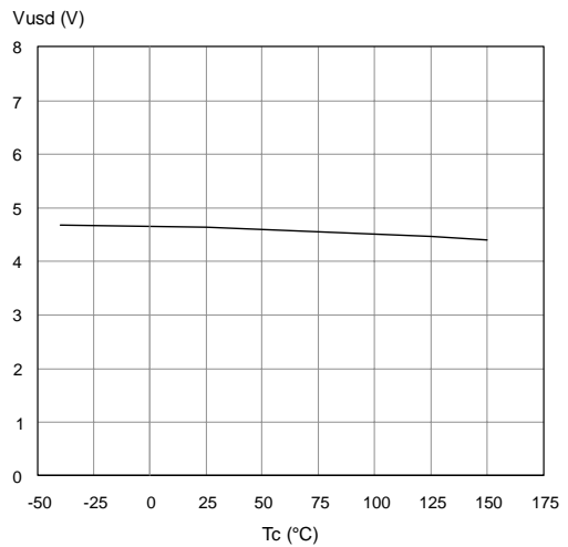
Figure 27. Undervoltage Shutdown
