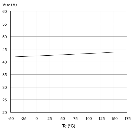
Figure 24. Overvoltage Shutdown
