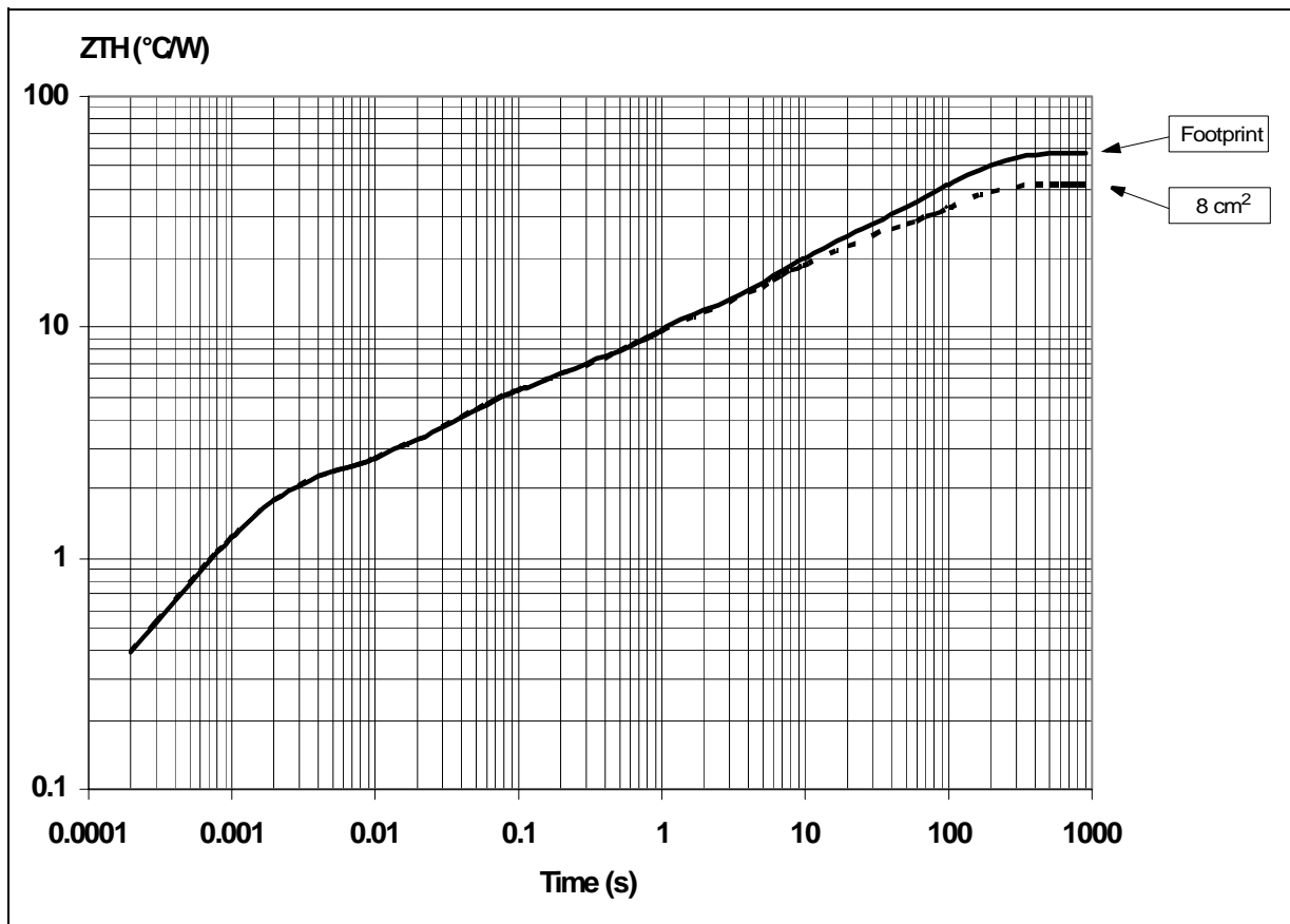
Figure 31. PowerSSO-24 Thermal Impedance Junction Ambient Single Pulse
