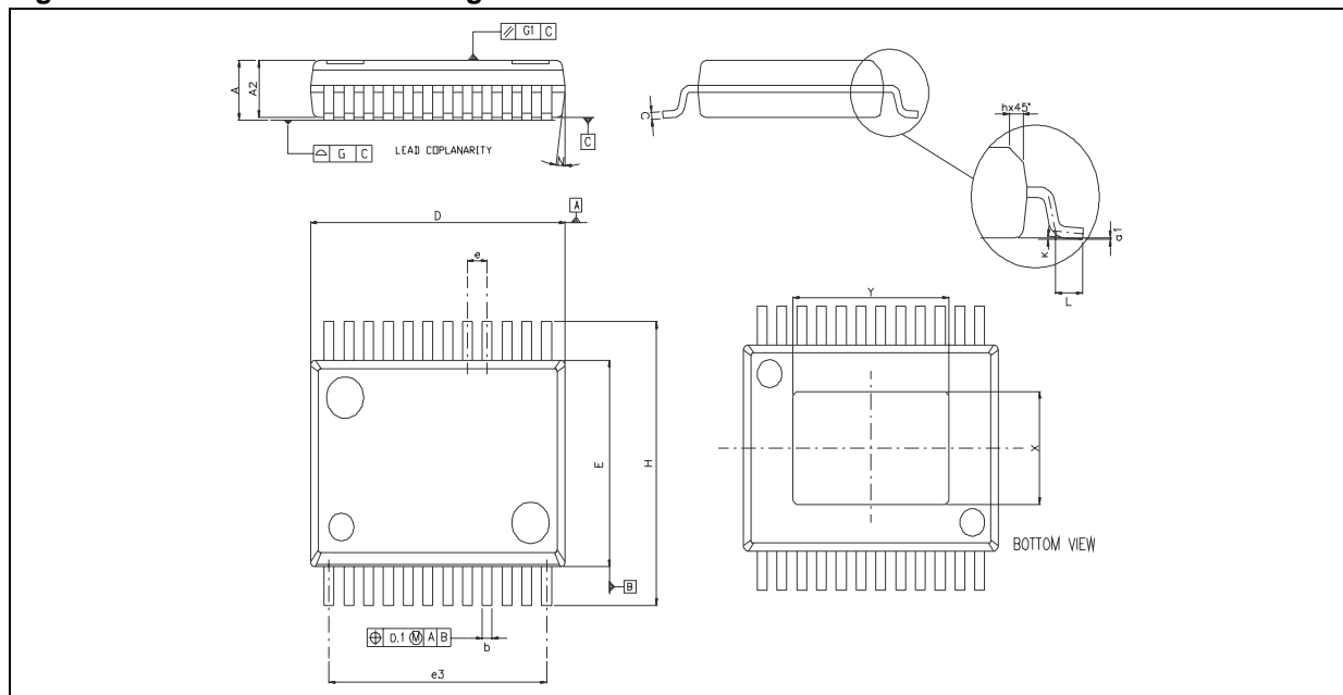
Figure 33. PowerSSO-24™ Package Dimensions
