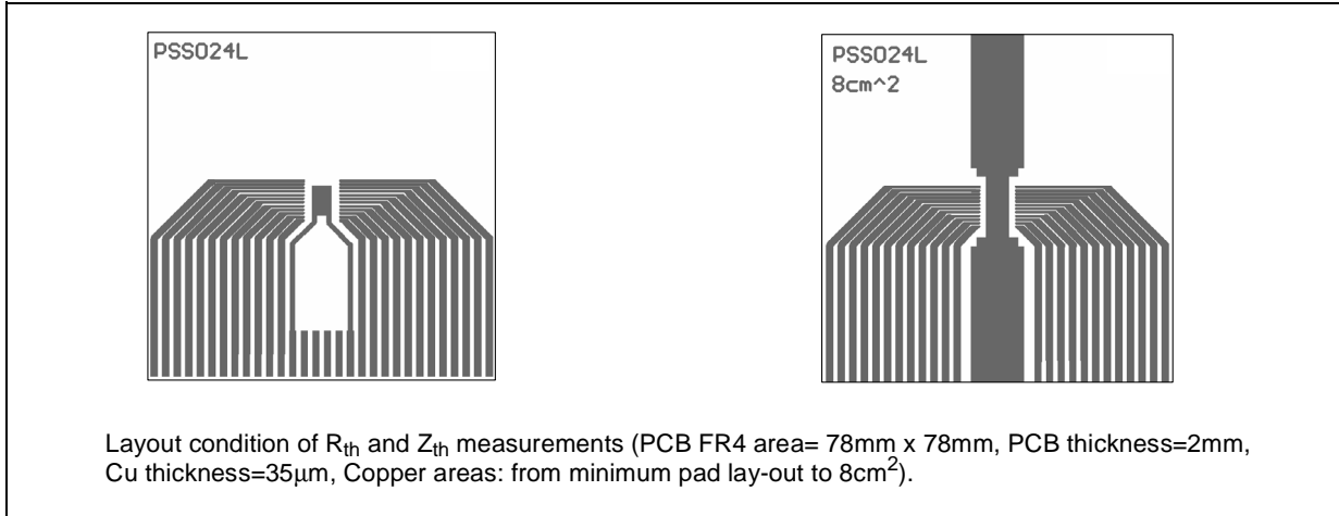
Figure 29. PowerSSO-24 PC Board
