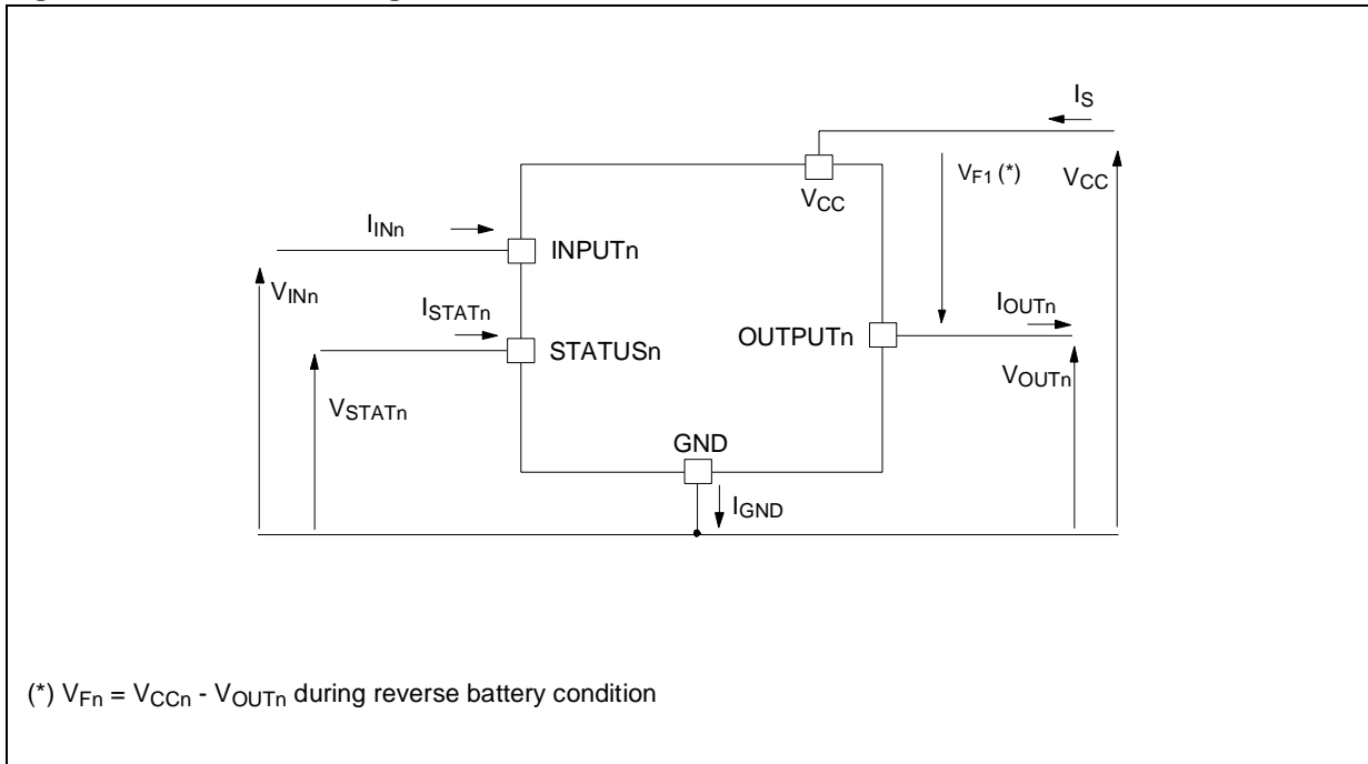
Figure 3. Current and Voltage Conventions
